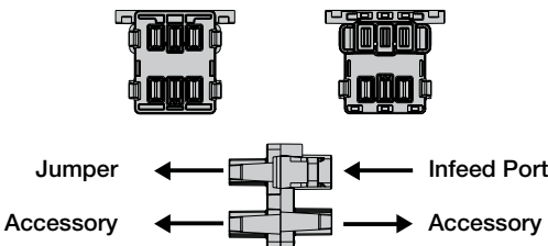
Accessory Distribution Block (Grey) BE07591-EF
